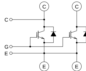
CIRCUIT DIAGRAM
